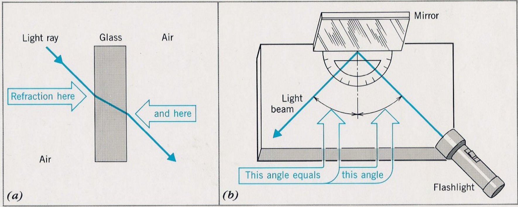
(a) The refraction light. (b) The reflection of light by a flat surface.
