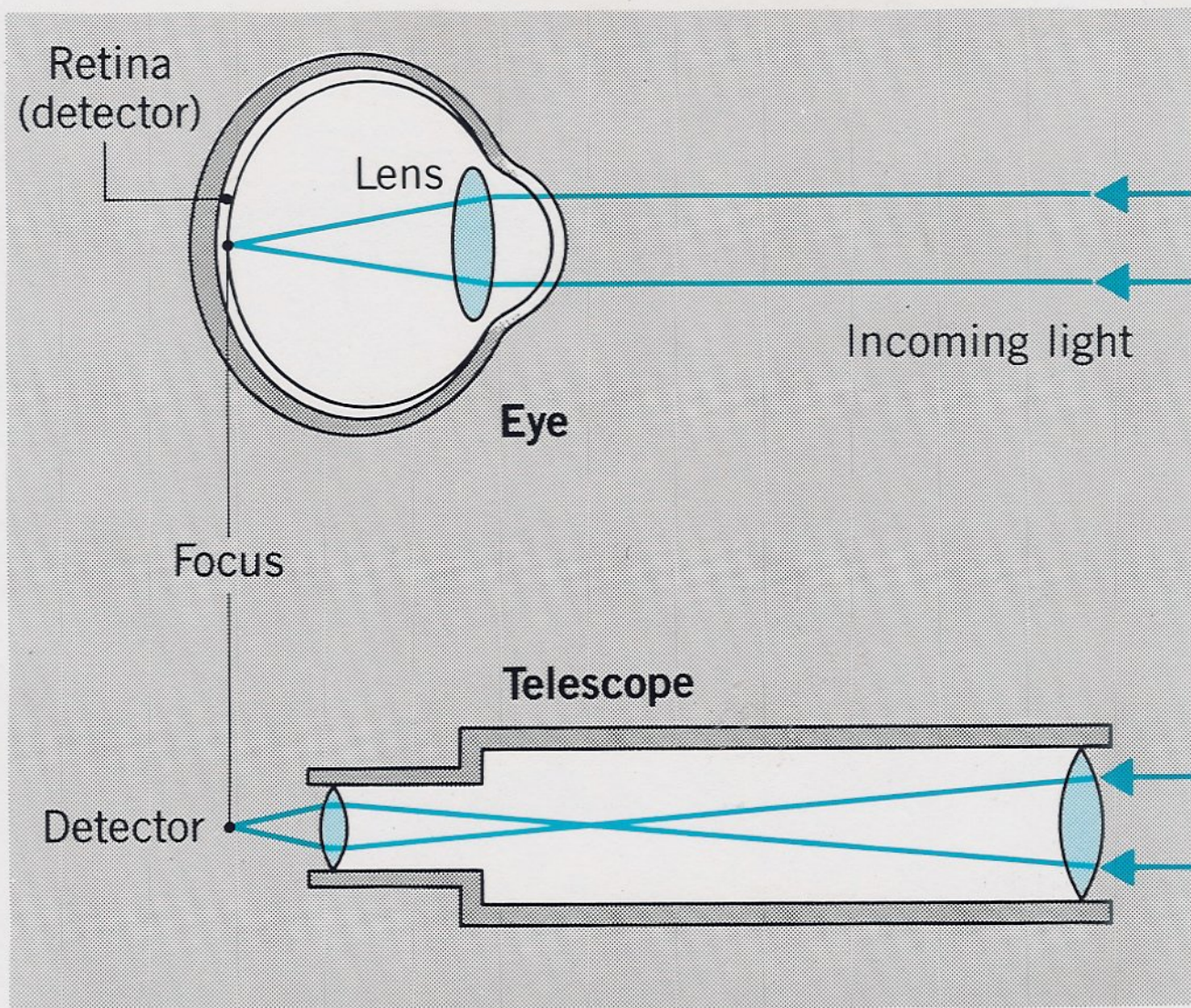
Comparison of the optics of the human eye (a) and a telescope (b).
