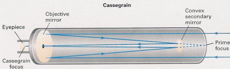
Pasachoff, Astronomy: From the Earth to the Universe, 6/e Figures 4.23, 4.13, 4.14, 4.16 and 4.17
